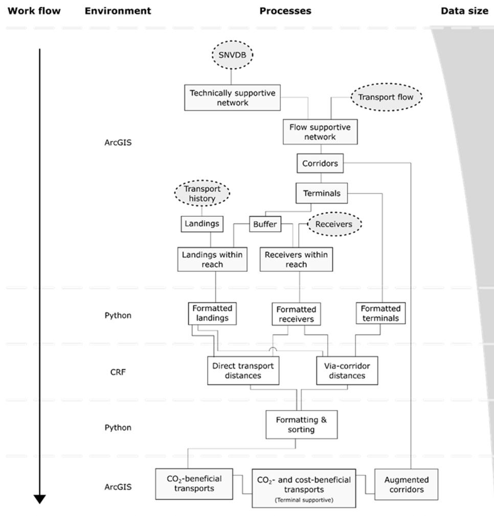
Figure 1. Schematic workflow of the study method, environment used, processes and data size. Ellipses are input data, rectangles are process-derived results.
